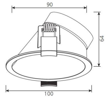
Asymmetrical Trim Ø95
